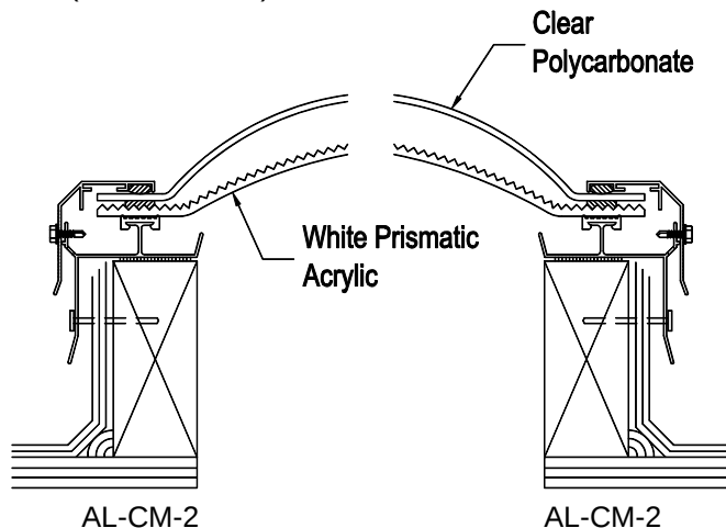
Polycarbonate/Prismatic Dome
